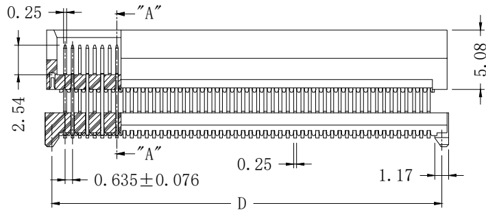
SECTION "B"-"B"
