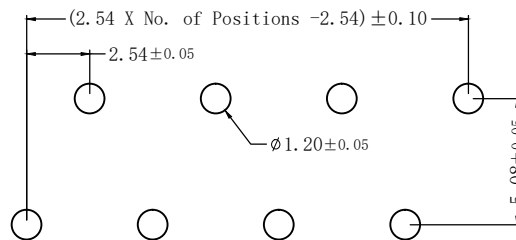
Recommended PCB Layout B2 Type
