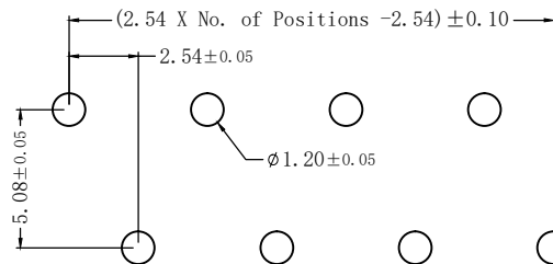
Recommended PCB Layout B1 Type
